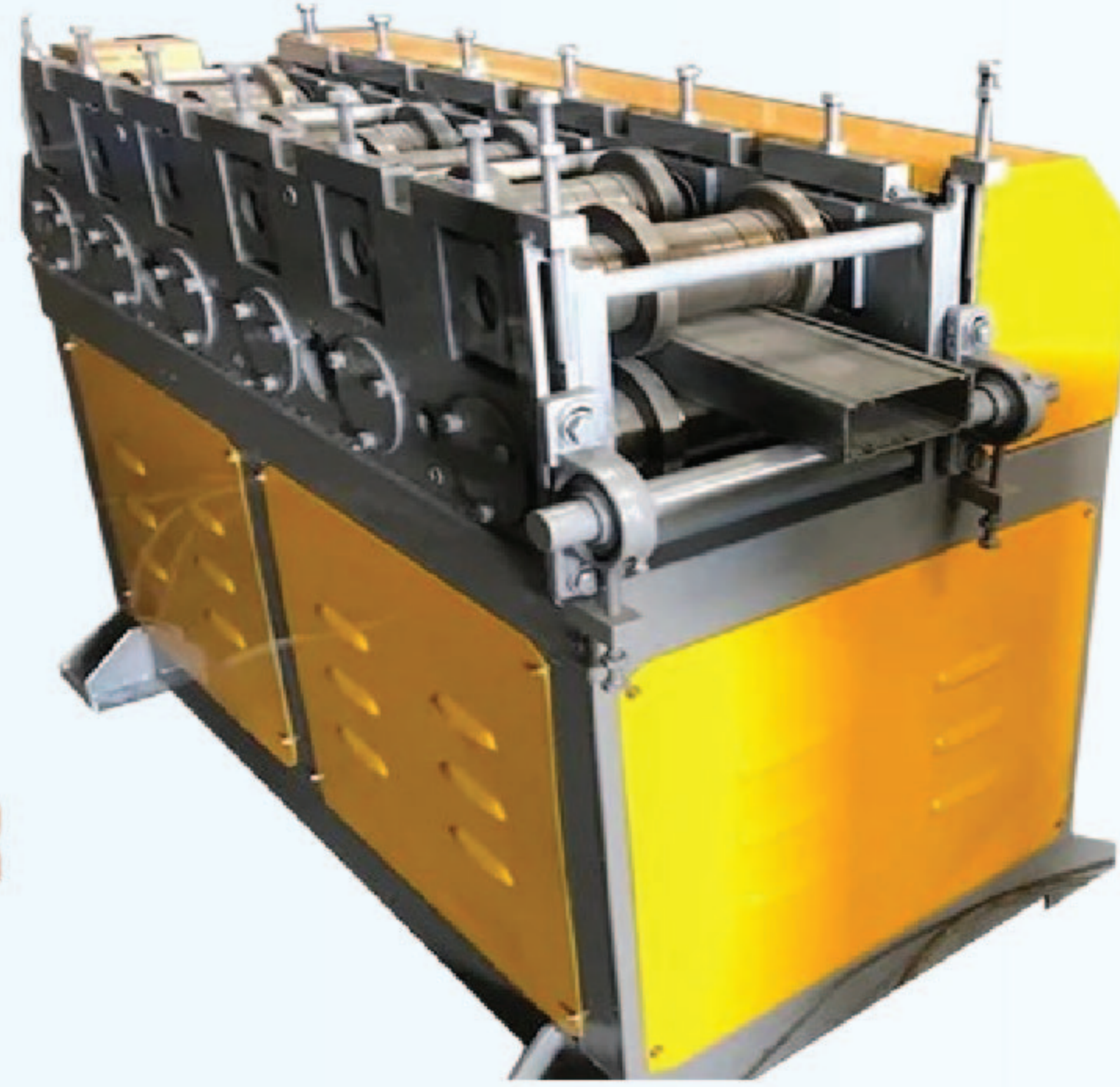
BEAM MACHINE
